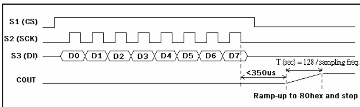
Fig. 11 Power-up command timing
