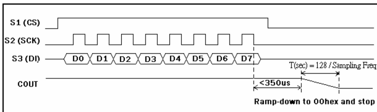
Fig. 12 Power-down commands timing
